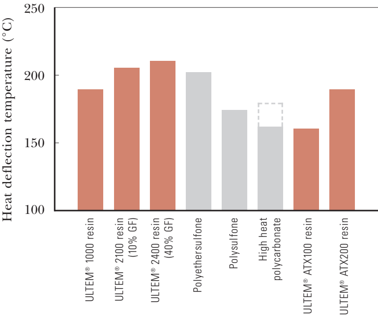
■ FIGURE 4-2 Heat Deflection Temperature (HDT/Ae 1.80 MPa)
